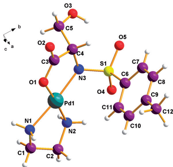
Figure 5. Molecular structure and atom-labeling scheme for 1 .
