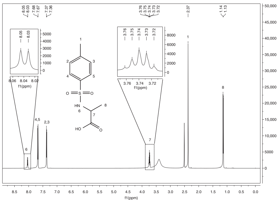
Figure 3. 1 H NMR spectra of TsalaH 2 in DMSO-d 6 .
